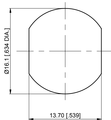
Recommend Mounting Hole
